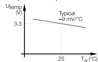
Temperature output
